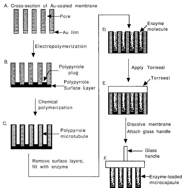
Figure 4. Schematic diagram of methods used to synthesize and enzyme-load the capsule arrays. (A) Au-coated template membrane. (B) Electropolymerization of polypyrrole film. (C) Chemical polymerization of polypyrrole tubules. (D) Loading with enzyme. (E) Capping with epoxy. (F) Dissolution of the template membrane.
