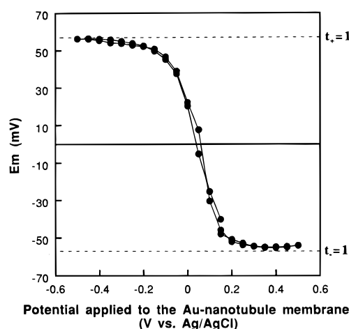
Figure 8. Variation of E_m with potential applied to the membrane (1 mM KF on the low-concentration (l) side, and 10 mM KF on the high concentration (h) side, of the membrane; tubule radius \sim 1.1 nm). The potential of the membrane was controlled with a potentiostat vs a Ag/AgCl reference electrode immersed in the side-h solution. E_m was measured with the membrane under potentiostatic control.
