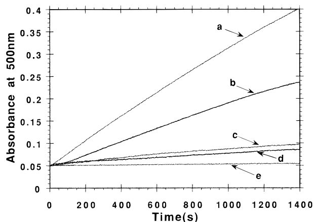
Figure 5. Evaluation of the enzymatic activity of GOx-loaded capsules (curves a and b) and empty capsules (curve e). The standard o -dianisidine/peroxidase assay was used. A larger amount of GOx was loaded into the capsules used for curve a than in the capsules used for curve b. Curves c and d are for a competing GOx-immobilization method—entrapment within a polypyrrole film.
