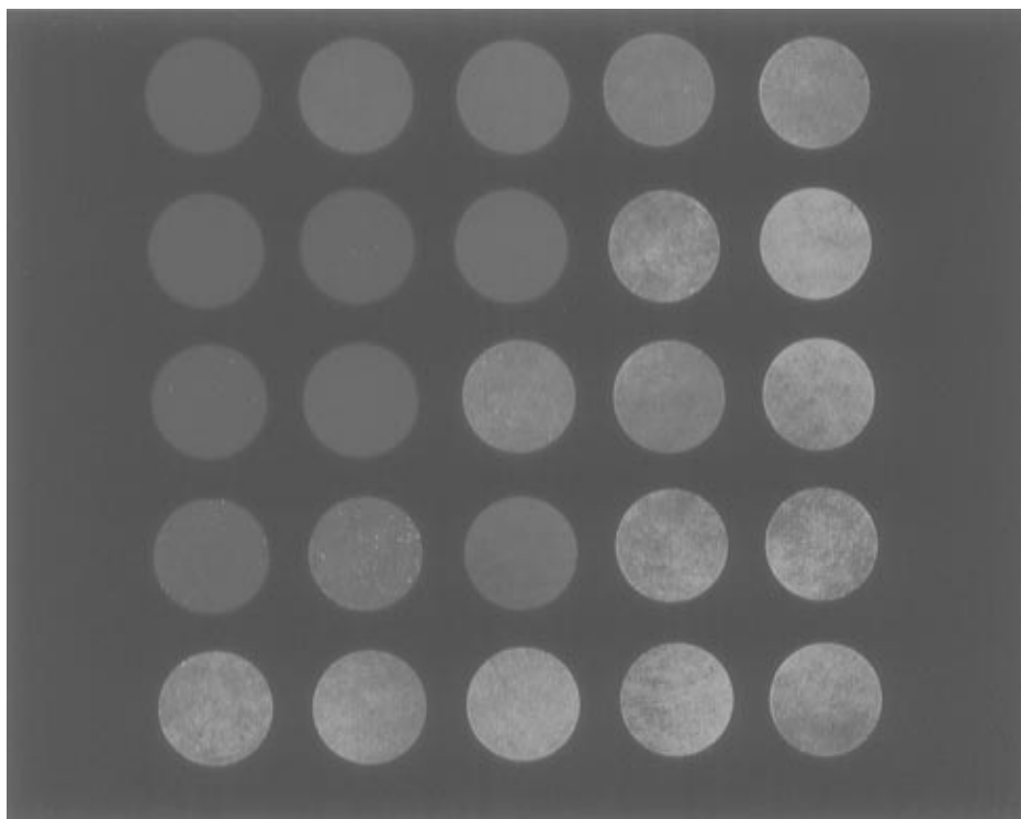
Figure 6. Photomicrographs (10 \times ) of pieces of the alumina membranes after deposition of gold fibrils of various aspect ratios into membranes with pores of various diameters. The diameters of the gold fibrils get smaller from the top row (150 nm diameter) to the bottom row (20 nm diameter). The aspect ratios of the gold fibrils get larger from left to right.
