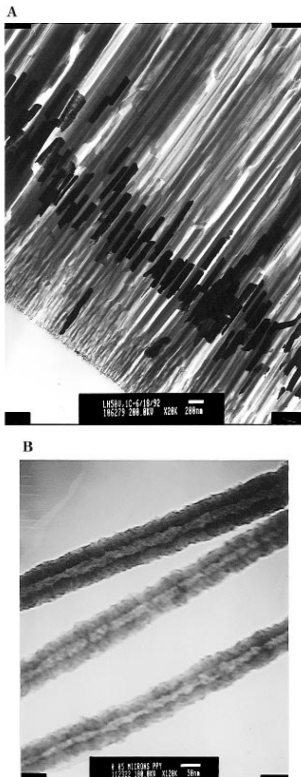
Figure 2. (A) Transmission electron micrograph of a microtomed section of an alumina template membrane showing 70 nm diameter Au nanofibrils within the pores. (B) Transmission electron micrograph of three polypyrrole nanotubules. The outside diameter is ~90 nm; the inside diameter is ~20–30 nm.
