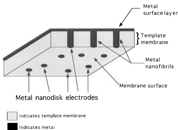
Figure 7. Schematic of an edge view of a nanoelectrode ensemble. The nanometal fibrils running through the pores of the template membrane are shown. The lower ends of the fibrils define nanodisks which are the electrodes. The opposite (upper) ends of the nanofibrils are connected to a common metal film, which is used to make electrical contact to the nanodisks. We have used this method to make nanoelectrode ensembles containing gold disks with diameters as small as 10 nm. 43
