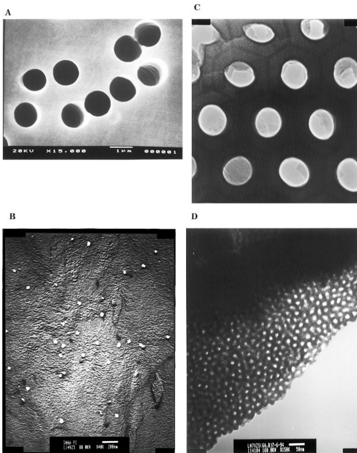
Figure 1. Electron micrographs of polycarbonate (A and B) and alumina (C and D) template membranes. For each type of membrane, an image of a larger pore membrane is presented (A and C) so that the characteristics of the pores can be clearly seen. An image of a membrane with extremely small pores is also presented (B and D). (A) Scanning electron micrograph of the surface of a polycarbonate membrane with 1 \mu\text{m} diameter pores. (B) Transmission electron micrograph (TEM) of a graphite replica of the surface of a polycarbonate membrane with 30 nm diameter pores. The pores appear "ragged". This is an artifact of the graphite replica. (C and D) TEMs of microtomed section of alumina membranes with 70 nm (C) and 10 nm (D) diameter pores.
